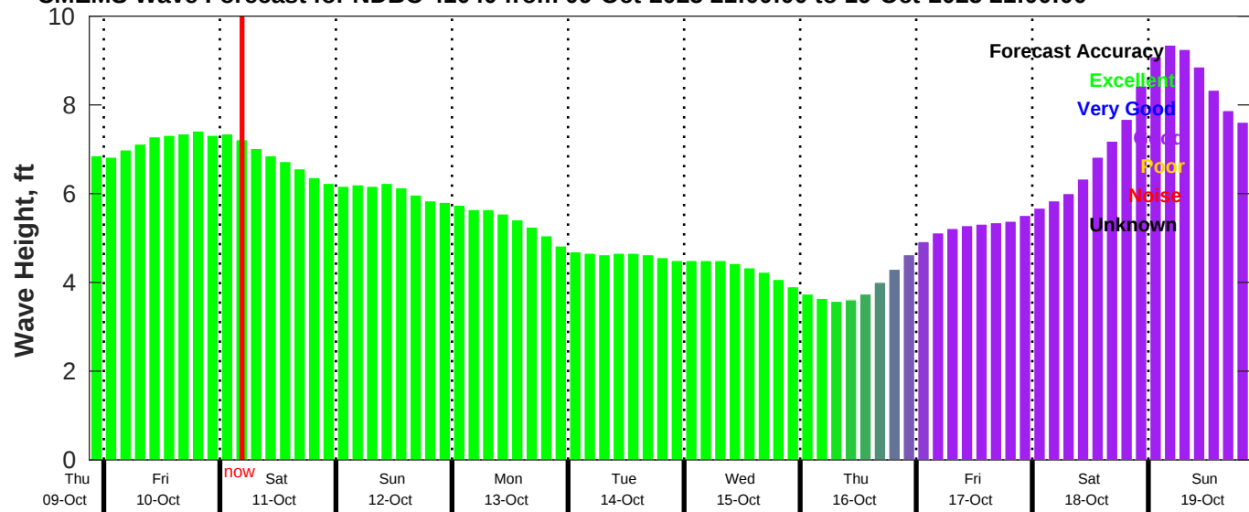
CMEMS Wave Forecast for NDBC 41040 from 09-Oct-2025 21:00:00 to 19-Oct-2025 21:00:00
