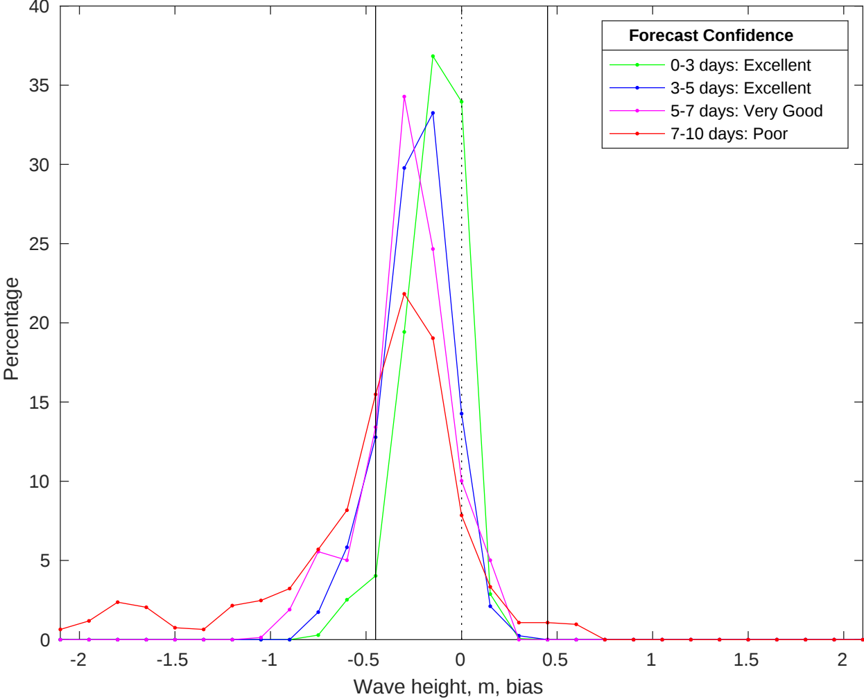
NDBC 42019 vs CMEMS Waves Bias Histogram: 11-Oct-2025
