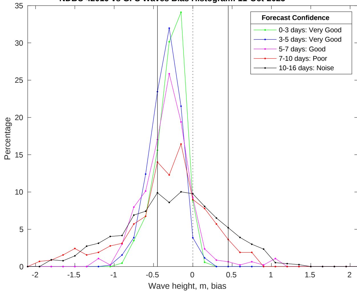
NDBC 42019 vs GFS Waves Bias Histogram: 11-Oct-2025
