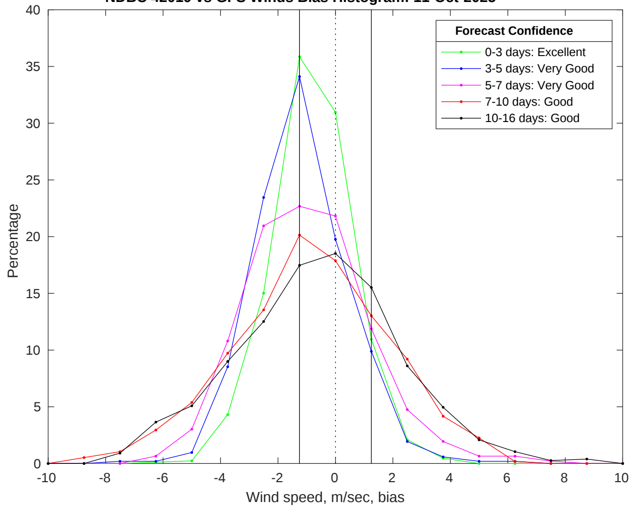
NDBC 42019 vs GFS Winds Bias Histogram: 11-Oct-2025
