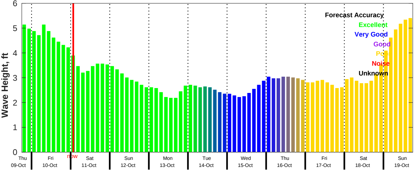
CMEMS Wave Forecast for NDBC 42019 from 09-Oct-2025 18:00:00 to 19-Oct-2025 18:00:00
