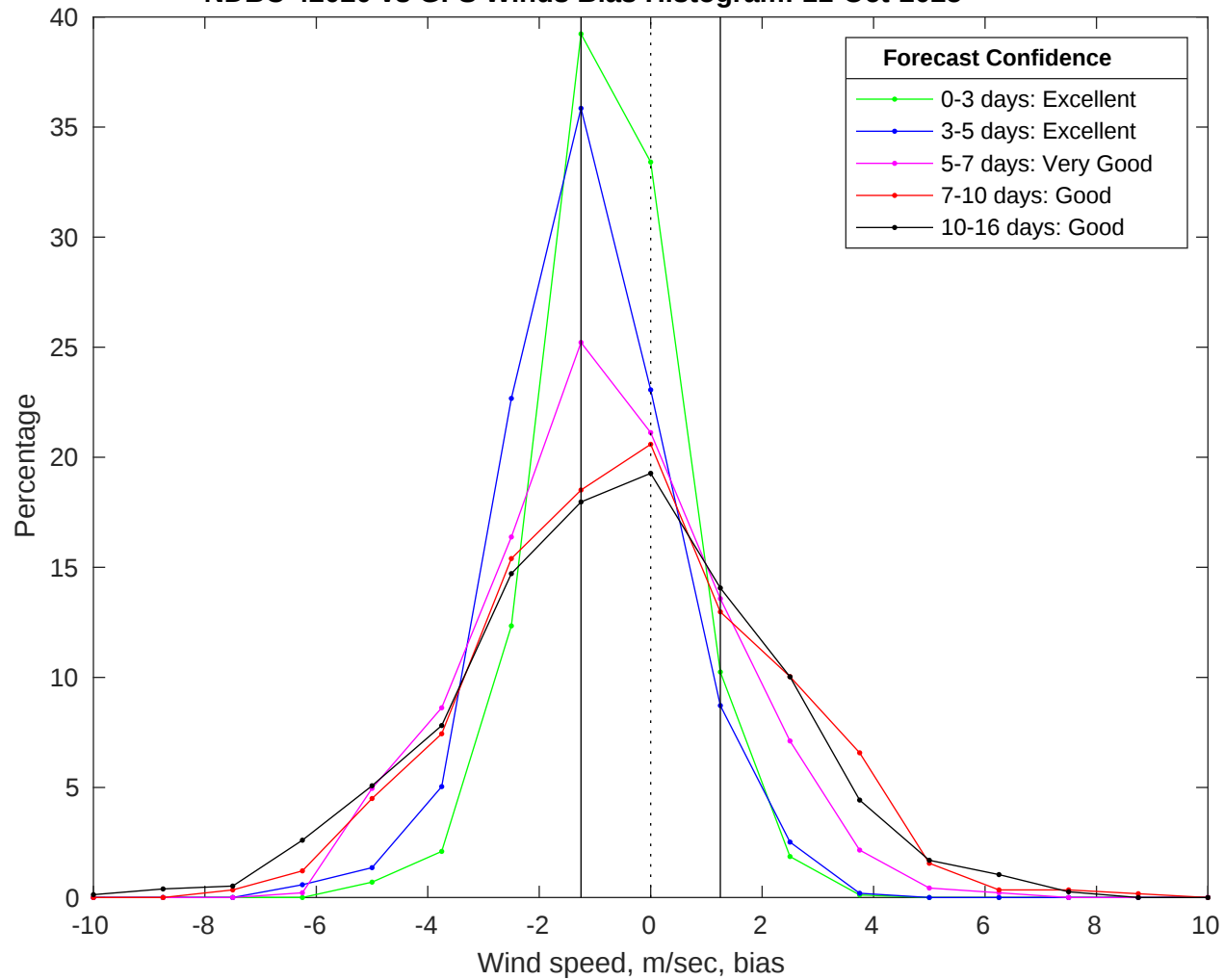
NDBC 42020 vs GFS Winds Bias Histogram: 11-Oct-2025
