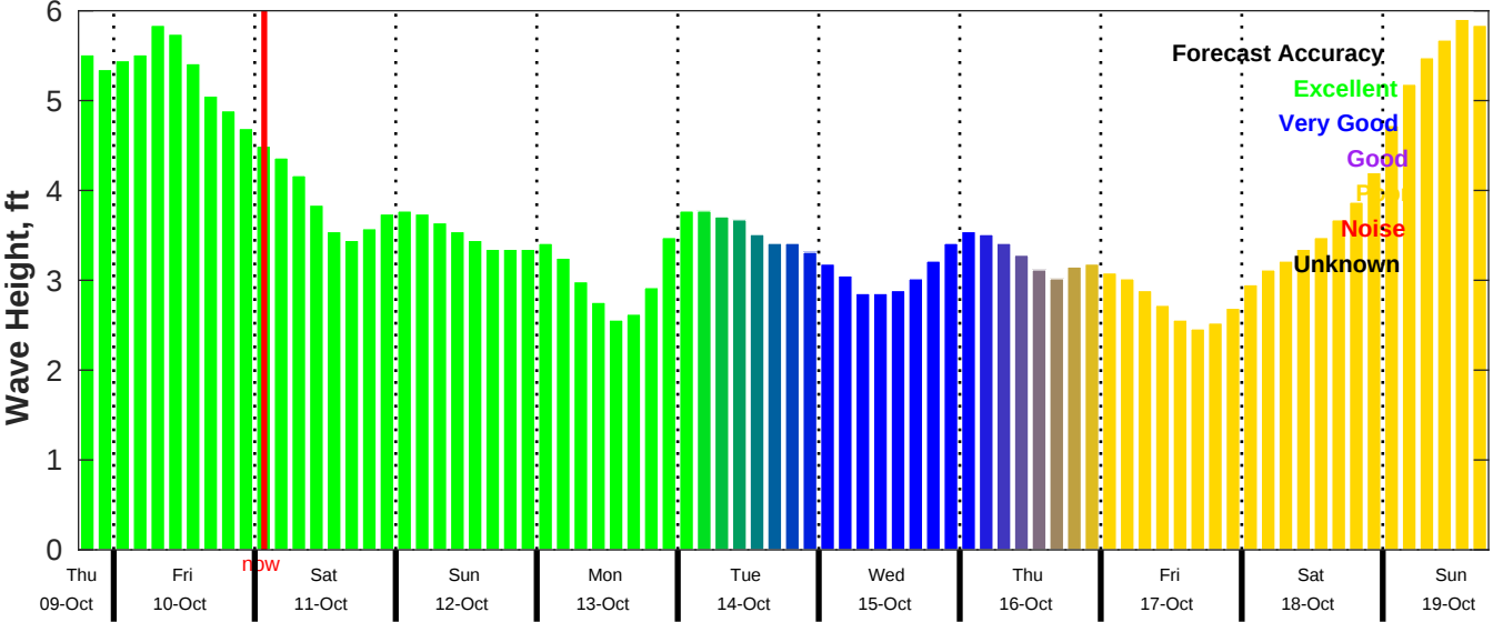
CMEMS Wave Forecast for NDBC 42020 from 09-Oct-2025 18:00:00 to 19-Oct-2025 18:00:00
