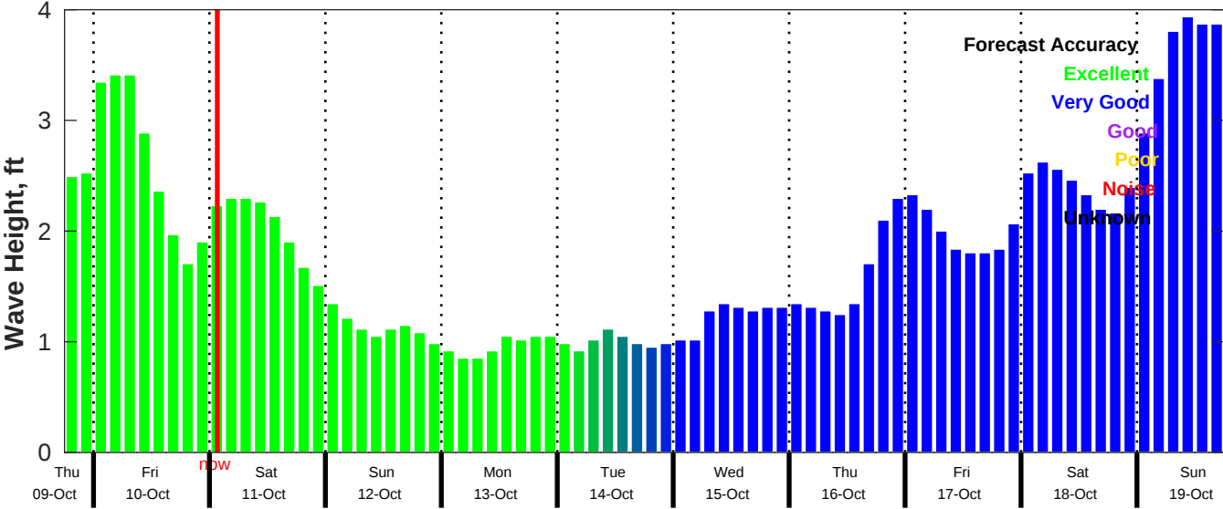
CMEMS Wave Forecast for NDBC 42035 from 09-Oct-2025 18:00:00 to 19-Oct-2025 18:00:00
