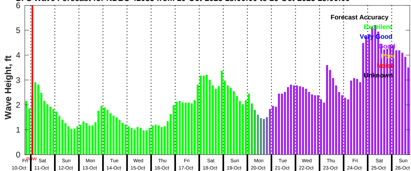
GFS Wave Forecast for NDBC 42035 from 10-Oct-2025 18:00:00 to 26-Oct-2025 18:00:00
