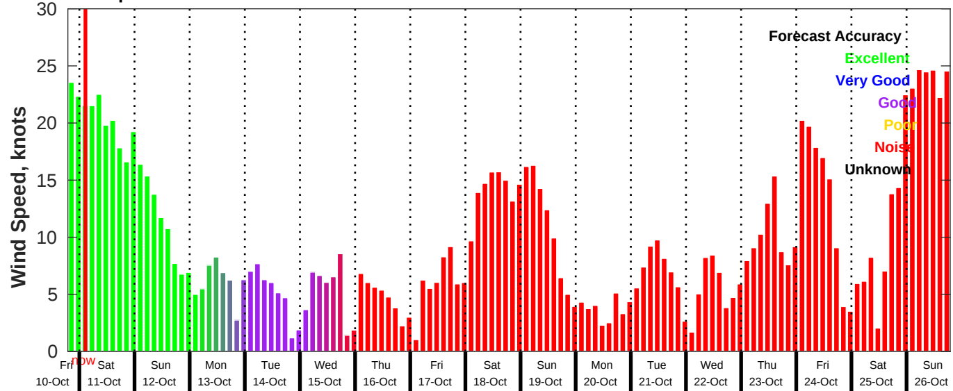
GFS Wind Speed Forecast for NDBC 42036 from 10-Oct-2025 19:00:00 to 26-Oct-2025 19:00:00
