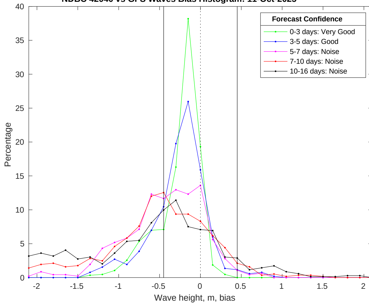
NDBC 42040 vs GFS Waves Bias Histogram: 11-Oct-2025
