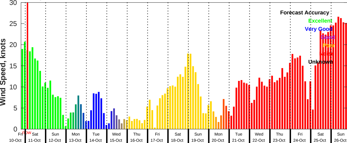
GFS Wind Speed Forecast for NDBC 42040 from 10-Oct-2025 19:00:00 to 26-Oct-2025 19:00:00
