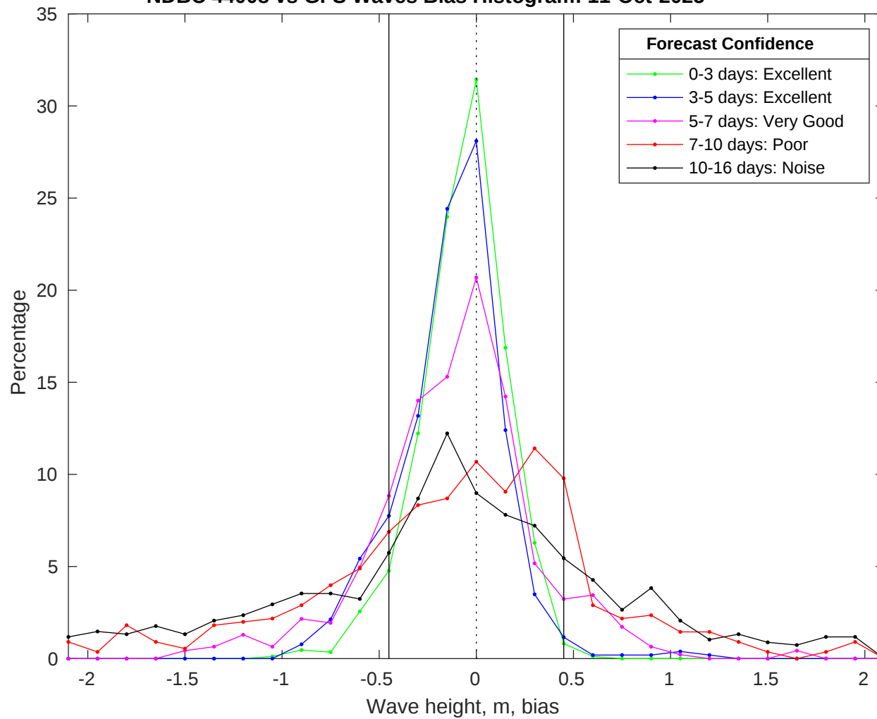
NDBC 44008 vs GFS Waves Bias Histogram: 11-Oct-2025
