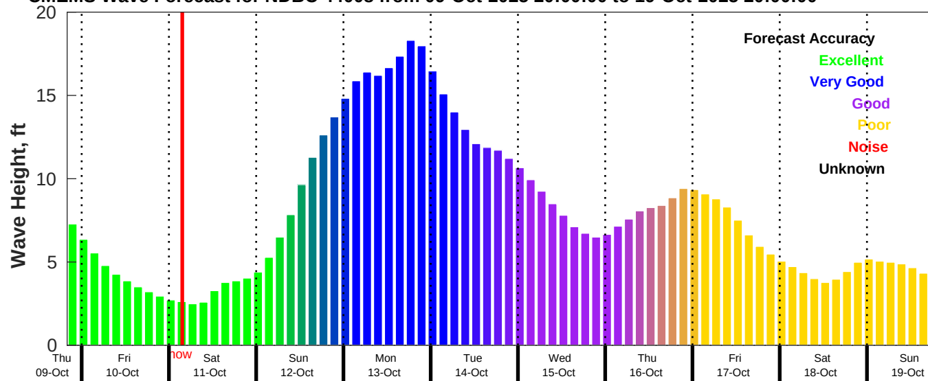
CMEMS Wave Forecast for NDBC 44008 from 09-Oct-2025 20:00:00 to 19-Oct-2025 20:00:00
