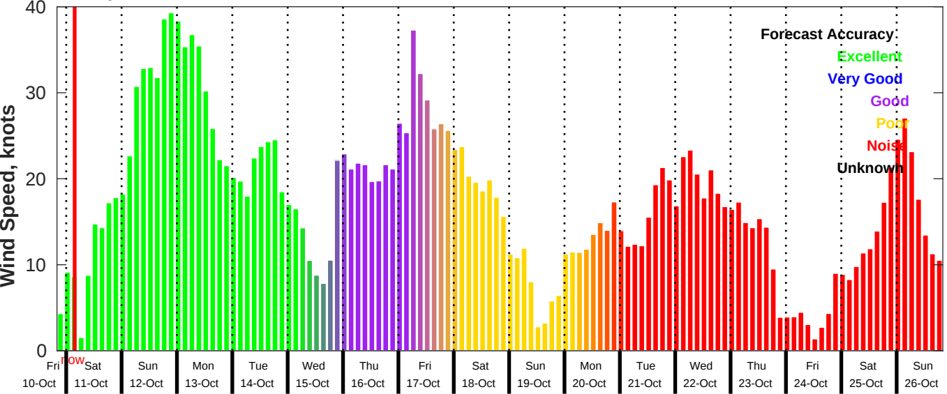
GFS Wind Speed Forecast for NDBC 44008 from 10-Oct-2025 20:00:00 to 26-Oct-2025 20:00:00
