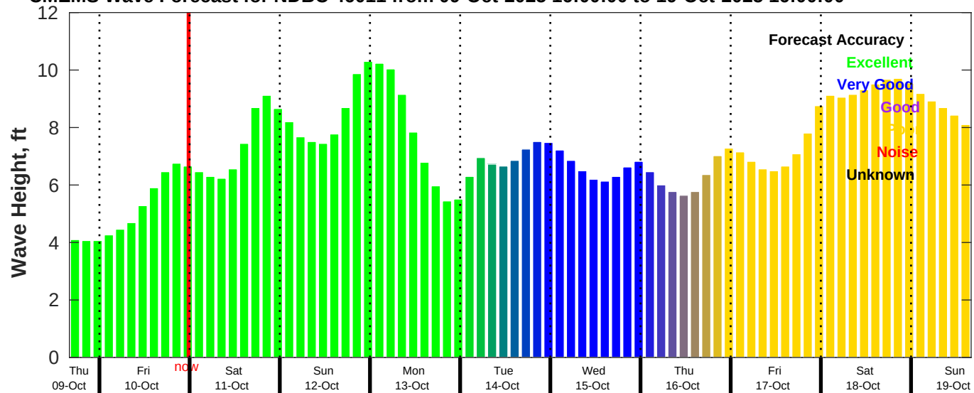
CMEMS Wave Forecast for NDBC 46011 from 09-Oct-2025 16:00:00 to 19-Oct-2025 16:00:00
