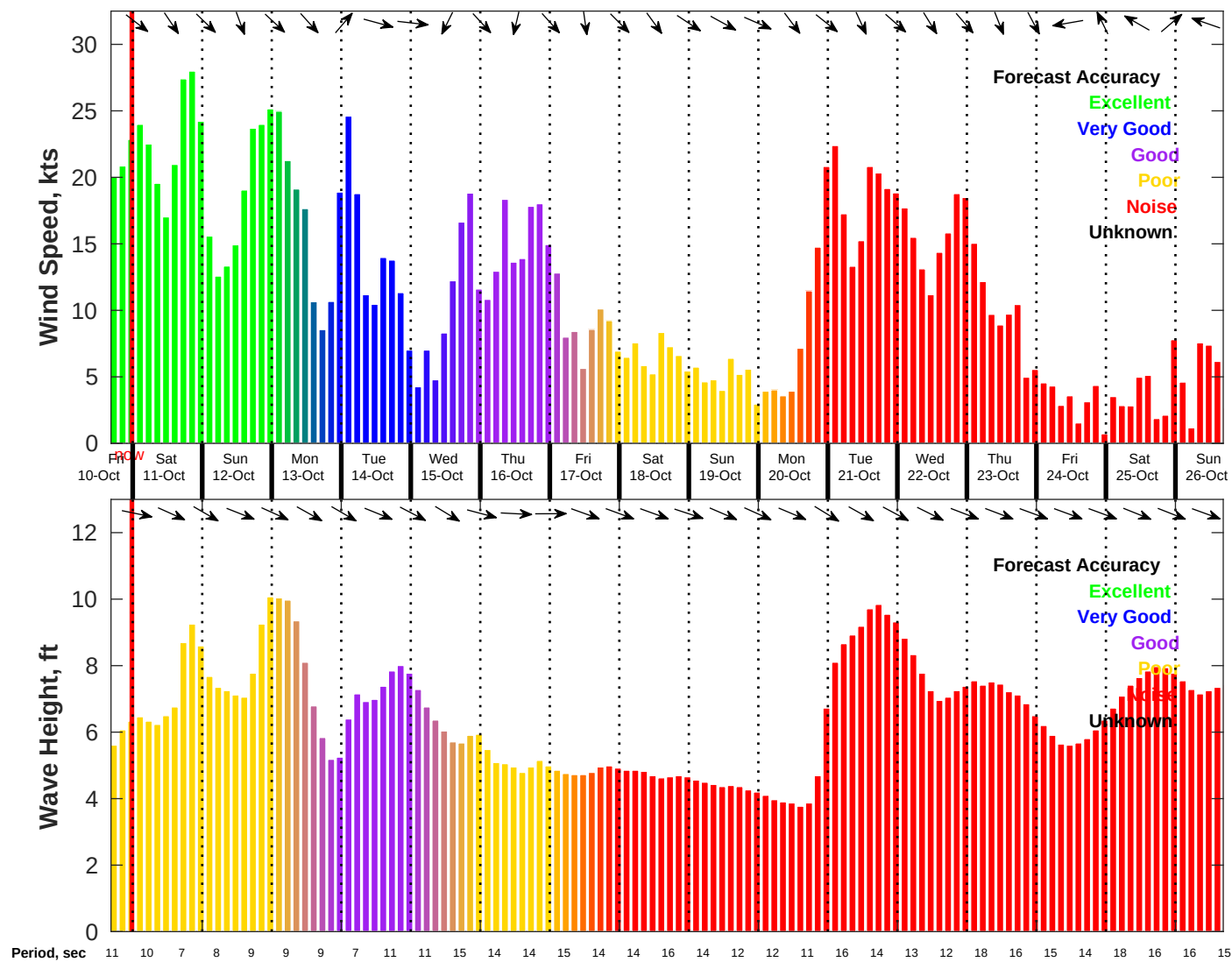
Wind & Wave Forecast for NDBC 46011 from 10-Oct-2025 16:00:00 to 26-Oct-2025 16:00:00
