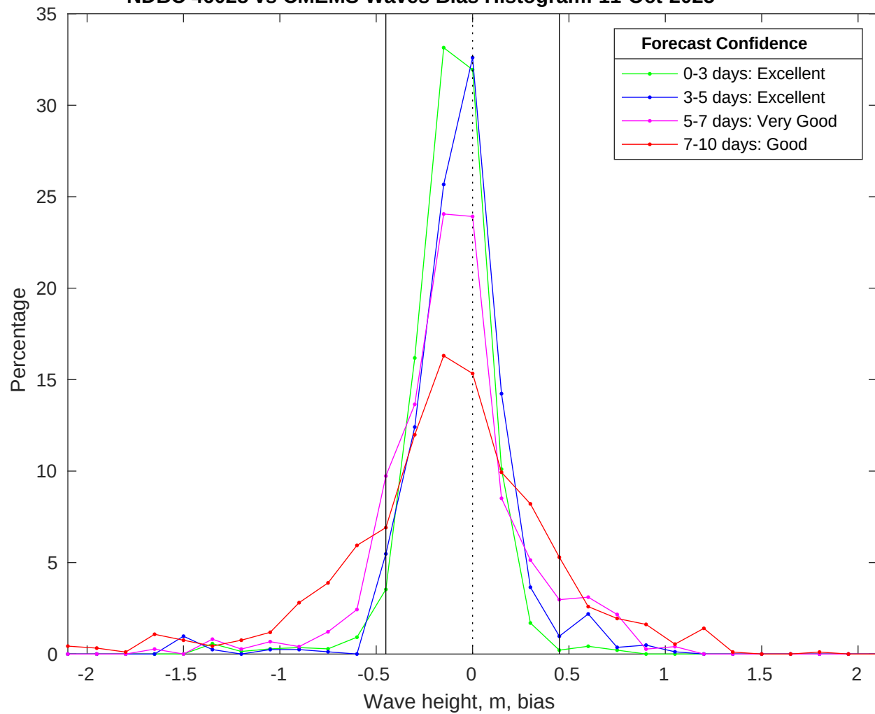
NDBC 46028 vs CMEMS Waves Bias Histogram: 11-Oct-2025
