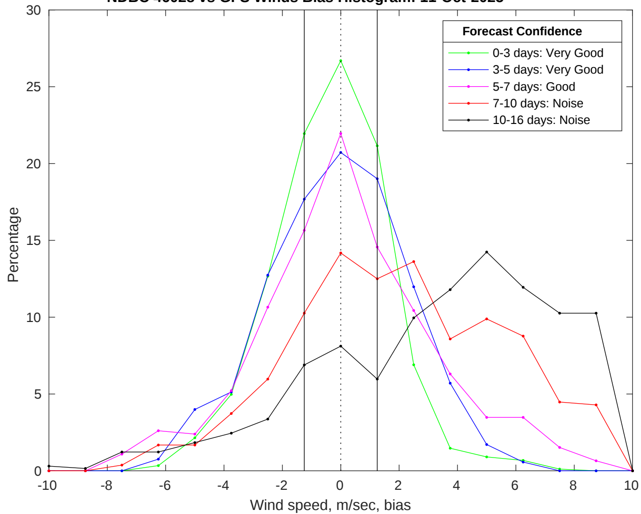
NDBC 46028 vs GFS Winds Bias Histogram: 11-Oct-2025
