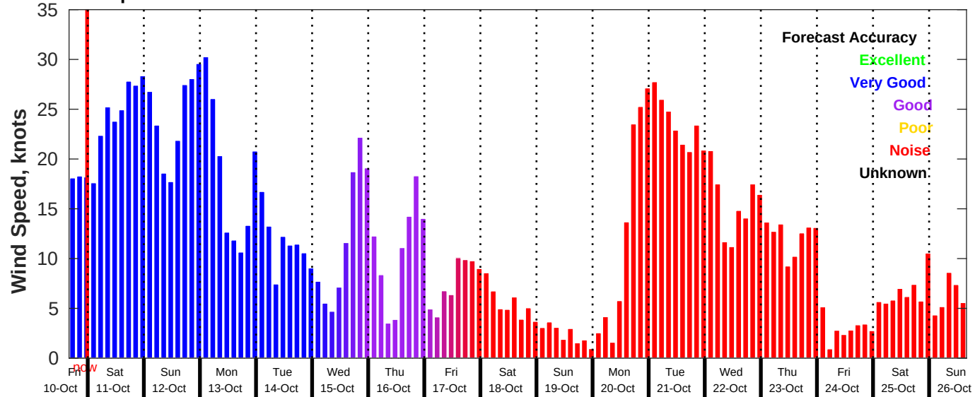
GFS Wind Speed Forecast for NDBC 46028 from 10-Oct-2025 16:00:00 to 26-Oct-2025 16:00:00
