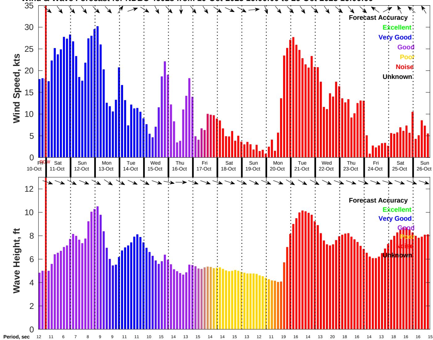
Wind & Wave Forecast for NDBC 46028 from 10-Oct-2025 16:00:00 to 26-Oct-2025 16:00:00
