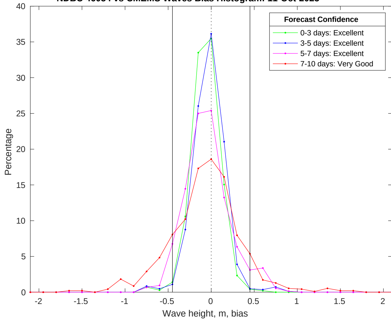
NDBC 46054 vs CMEMS Waves Bias Histogram: 11-Oct-2025
