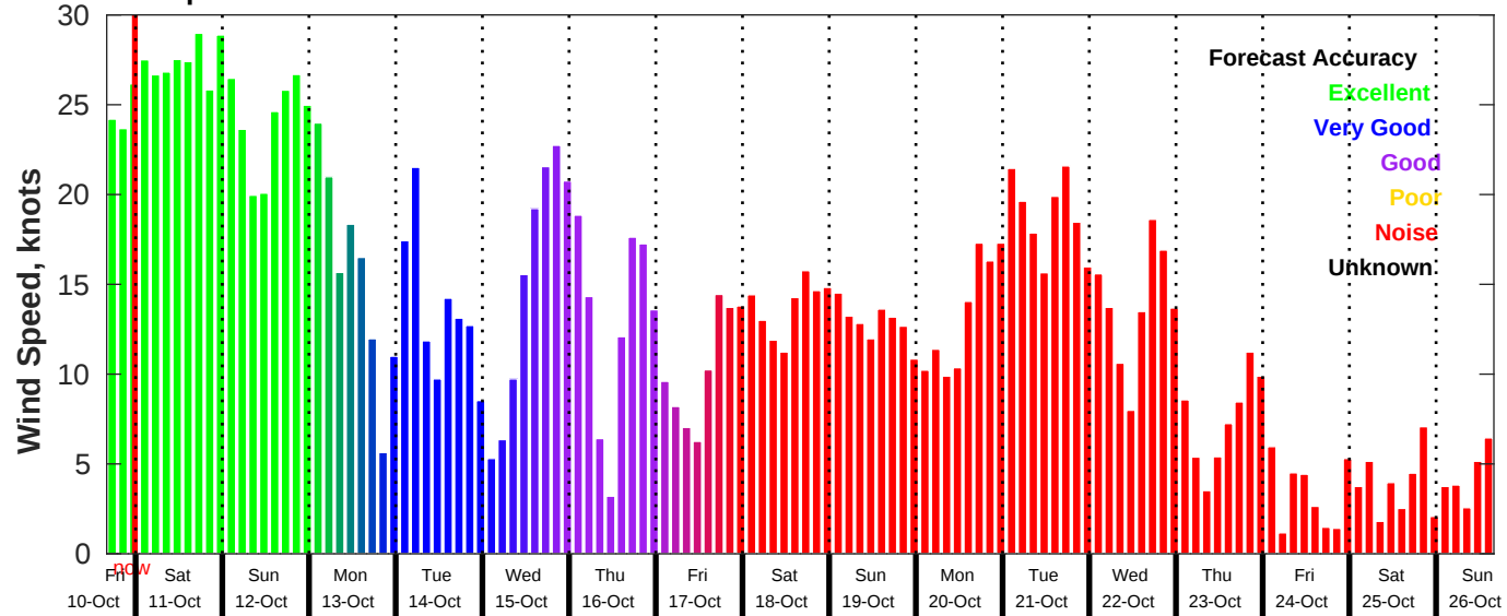
GFS Wind Speed Forecast for NDBC 46054 from 10-Oct-2025 16:00:00 to 26-Oct-2025 16:00:00
