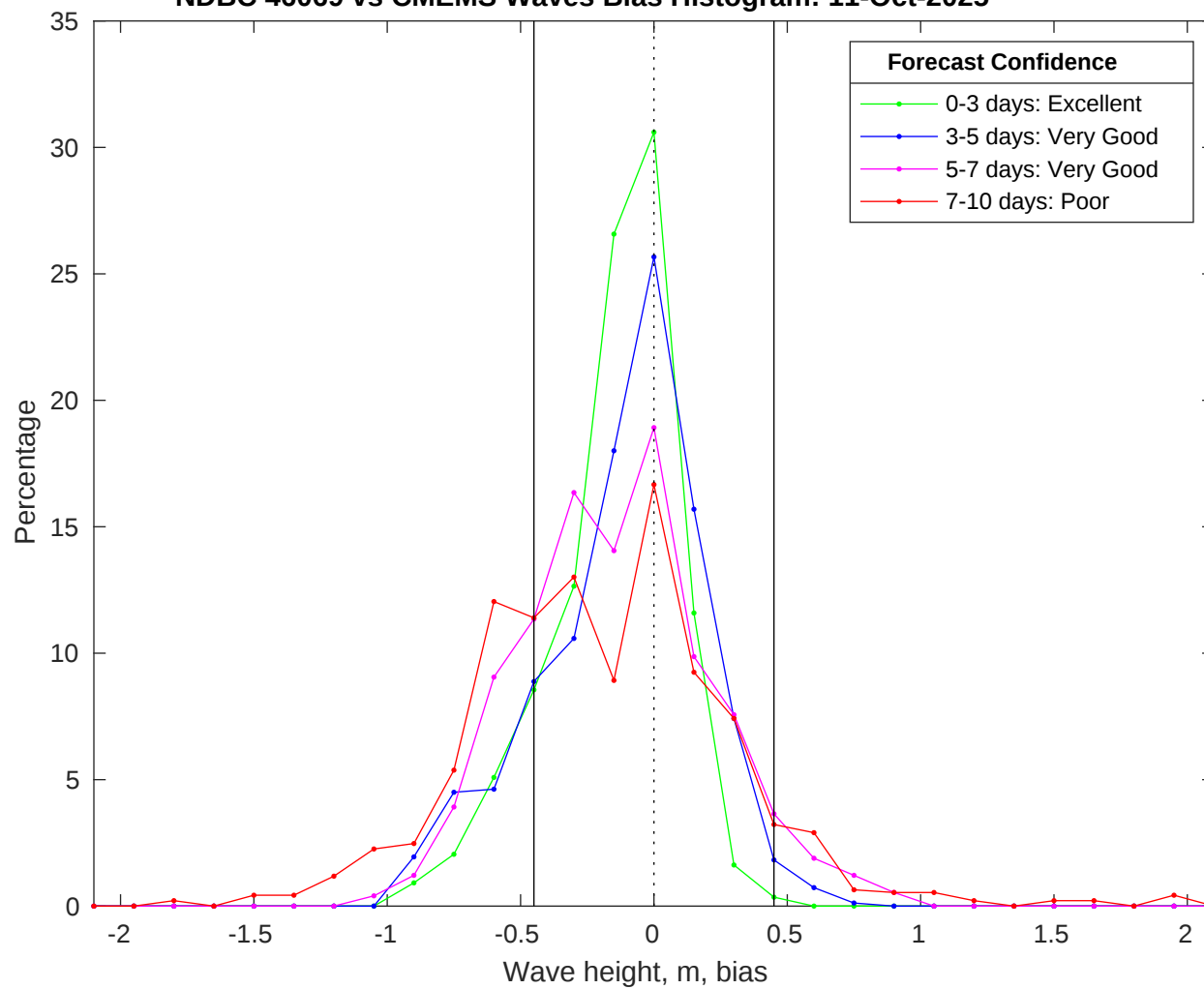
NDBC 46069 vs CMEMS Waves Bias Histogram: 11-Oct-2025
