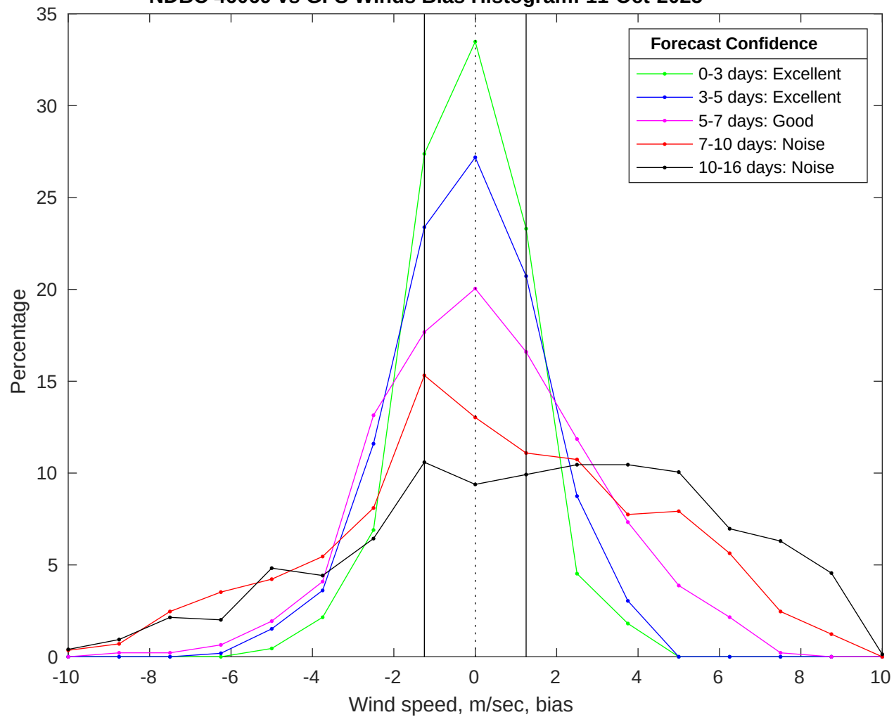
NDBC 46069 vs GFS Winds Bias Histogram: 11-Oct-2025
