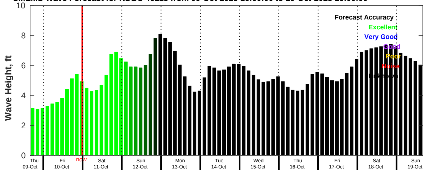
CMEMS Wave Forecast for NDBC 46215 from 09-Oct-2025 16:00:00 to 19-Oct-2025 16:00:00
