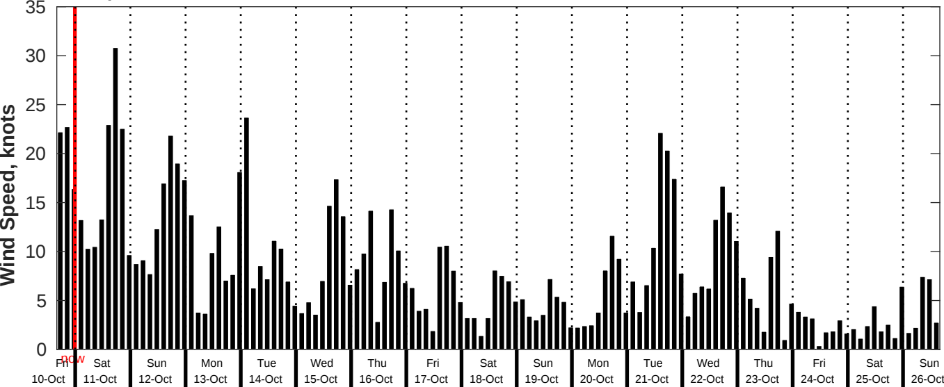
GFS Wind Speed Forecast for NDBC 46215 from 10-Oct-2025 16:00:00 to 26-Oct-2025 16:00:00
