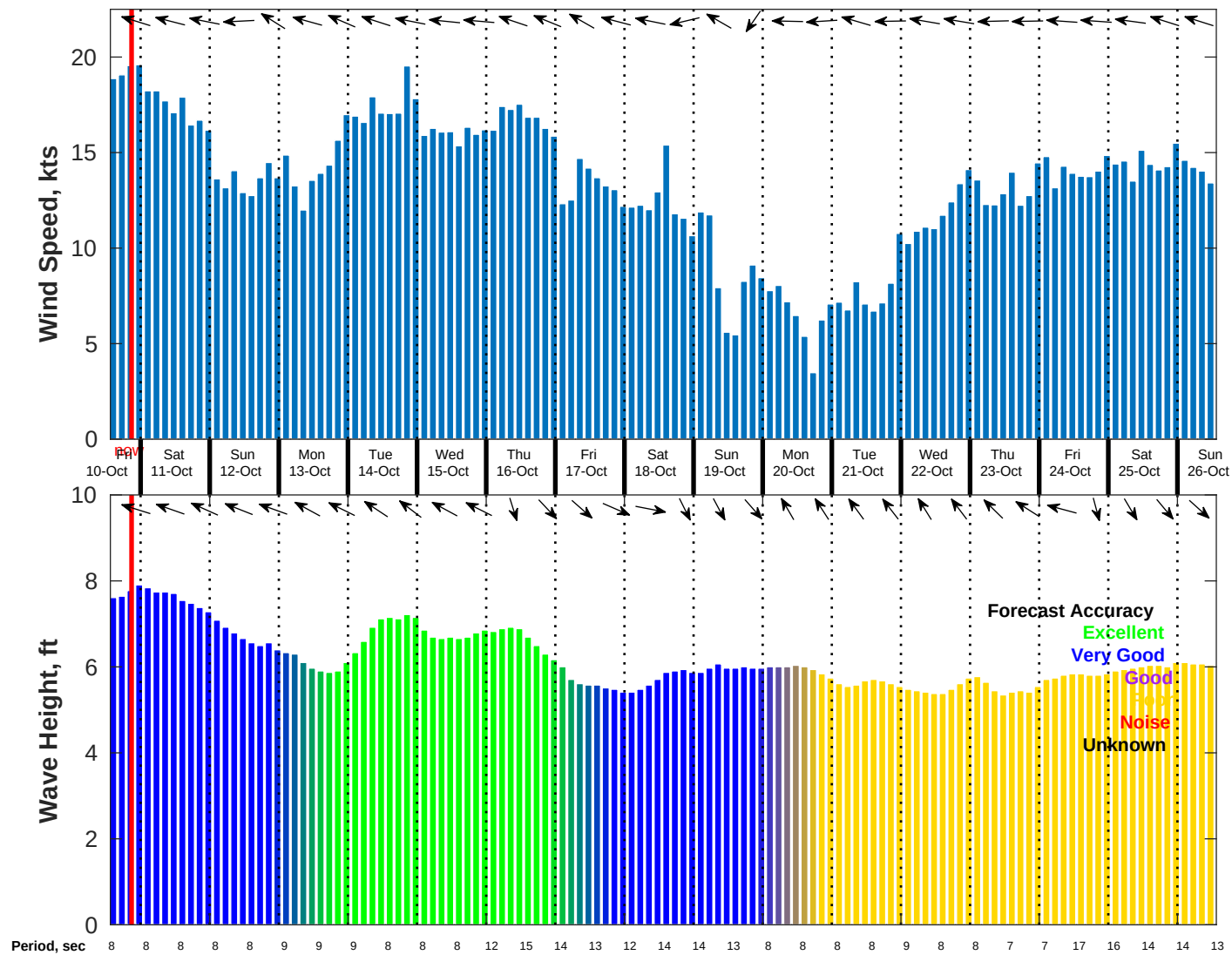
Wind & Wave Forecast for NDBC 51209 from 10-Oct-2025 13:00:00 to 26-Oct-2025 13:00:00
