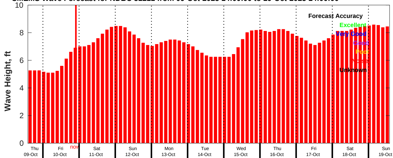
CMEMS Wave Forecast for NDBC 51211 from 09-Oct-2025 14:00:00 to 19-Oct-2025 14:00:00
