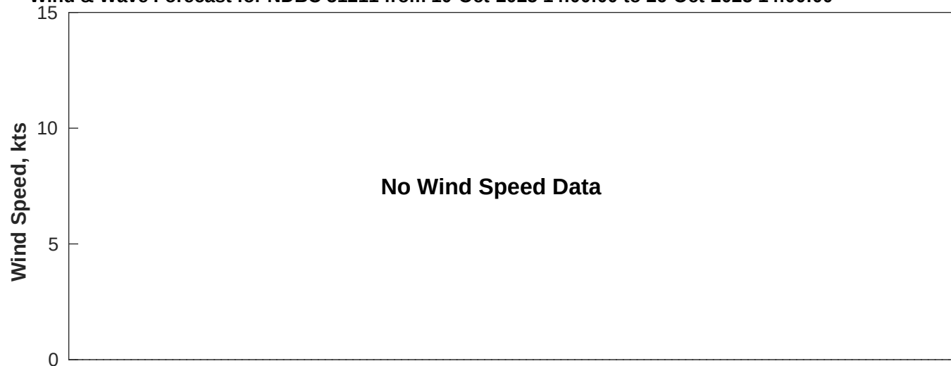
Wind & Wave Forecast for NDBC 51211 from 10-Oct-2025 14:00:00 to 26-Oct-2025 14:00:00
