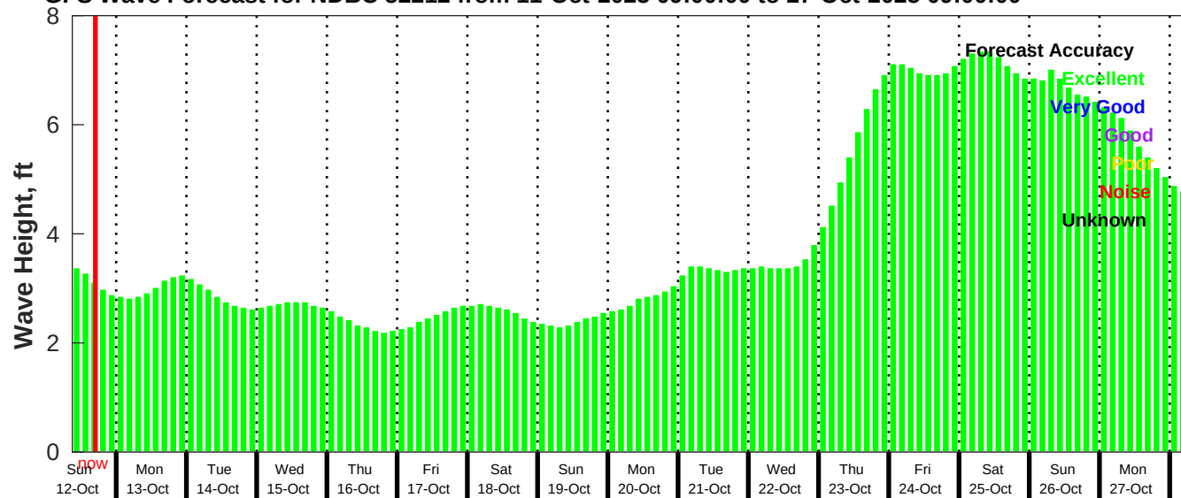
GFS Wave Forecast for NDBC 52212 from 11-Oct-2025 09:00:00 to 27-Oct-2025 09:00:00
