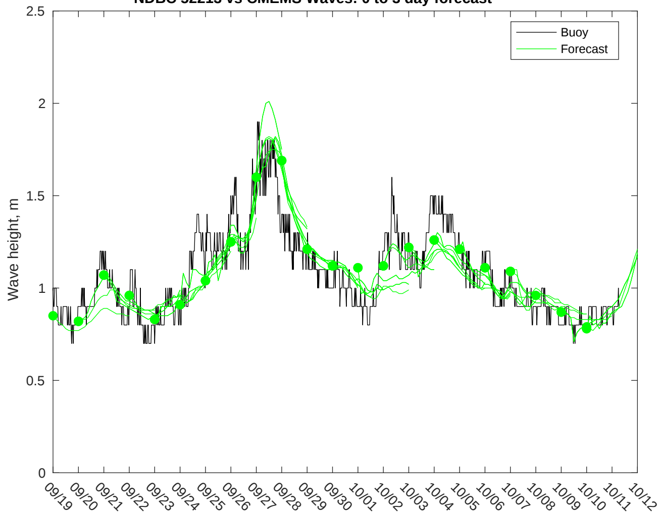
NDBC 52213 vs CMEMS Waves: 0 to 3 day forecast
