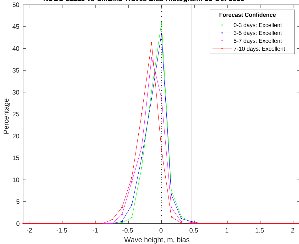
NDBC 52213 vs CMEMS Waves Bias Histogram: 11-Oct-2025
