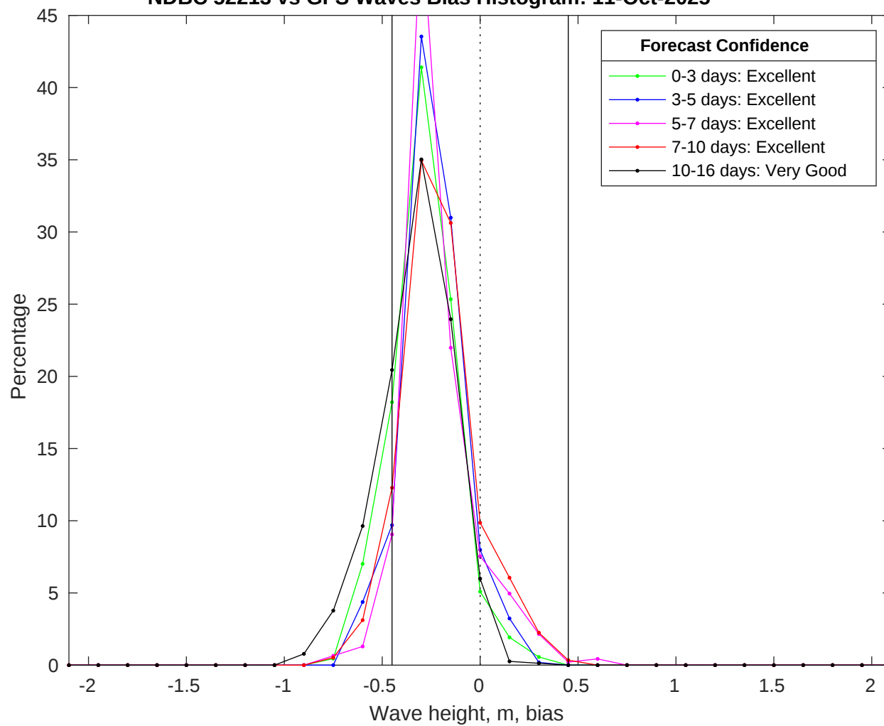
NDBC 52213 vs GFS Waves Bias Histogram: 11-Oct-2025
