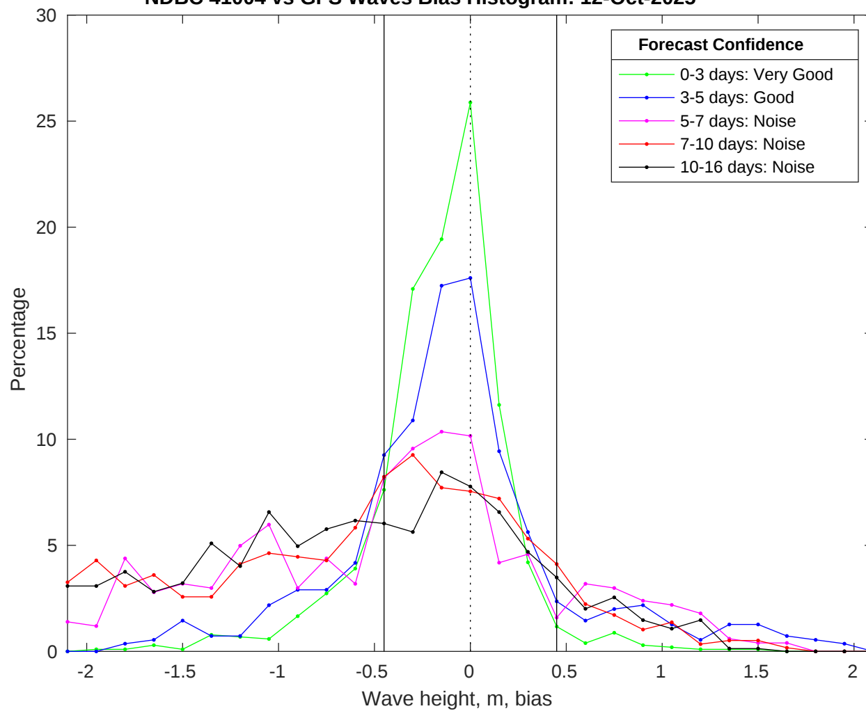
NDBC 41004 vs GFS Waves Bias Histogram: 12-Oct-2025
