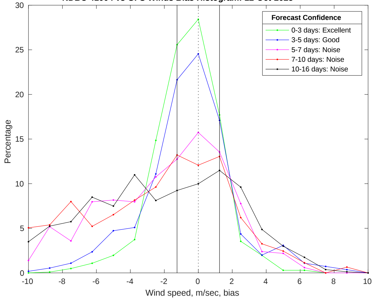
NDBC 41004 vs GFS Winds Bias Histogram: 12-Oct-2025
