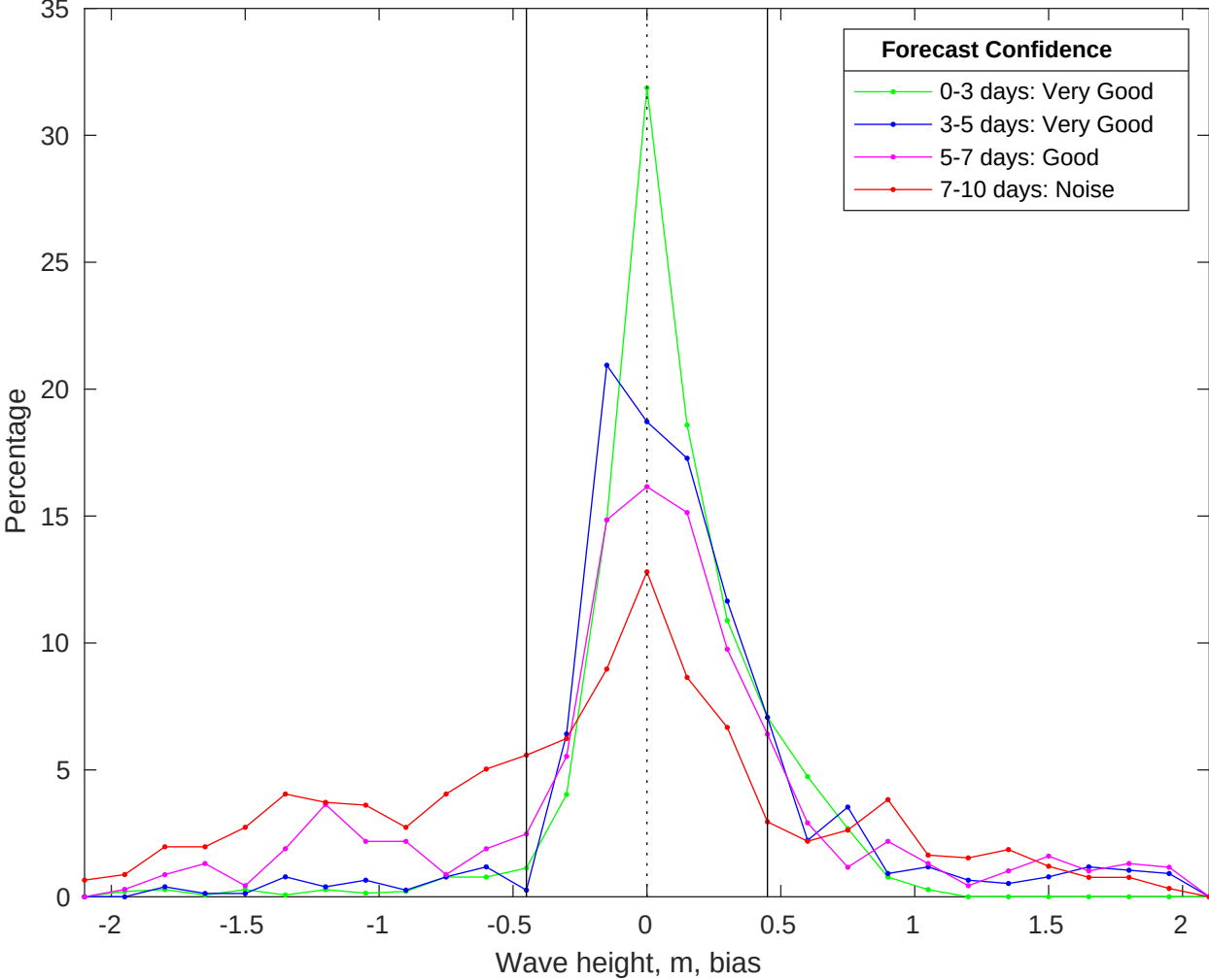
NDBC 41013 vs CMEMS Waves Bias Histogram: 12-Oct-2025
