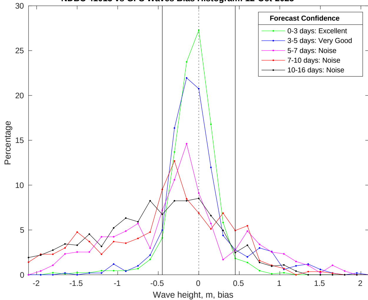
NDBC 41013 vs GFS Waves Bias Histogram: 12-Oct-2025
