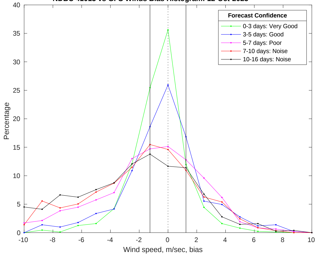
NDBC 41013 vs GFS Winds Bias Histogram: 12-Oct-2025
