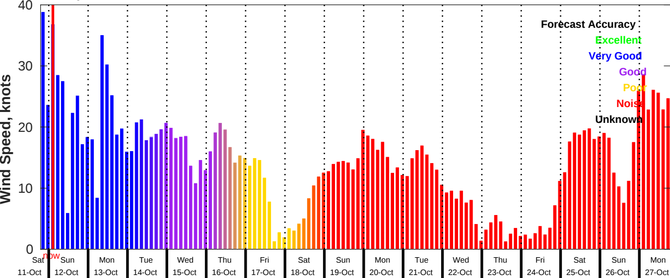
GFS Wind Speed Forecast for NDBC 41013 from 11-Oct-2025 19:00:00 to 27-Oct-2025 19:00:00
