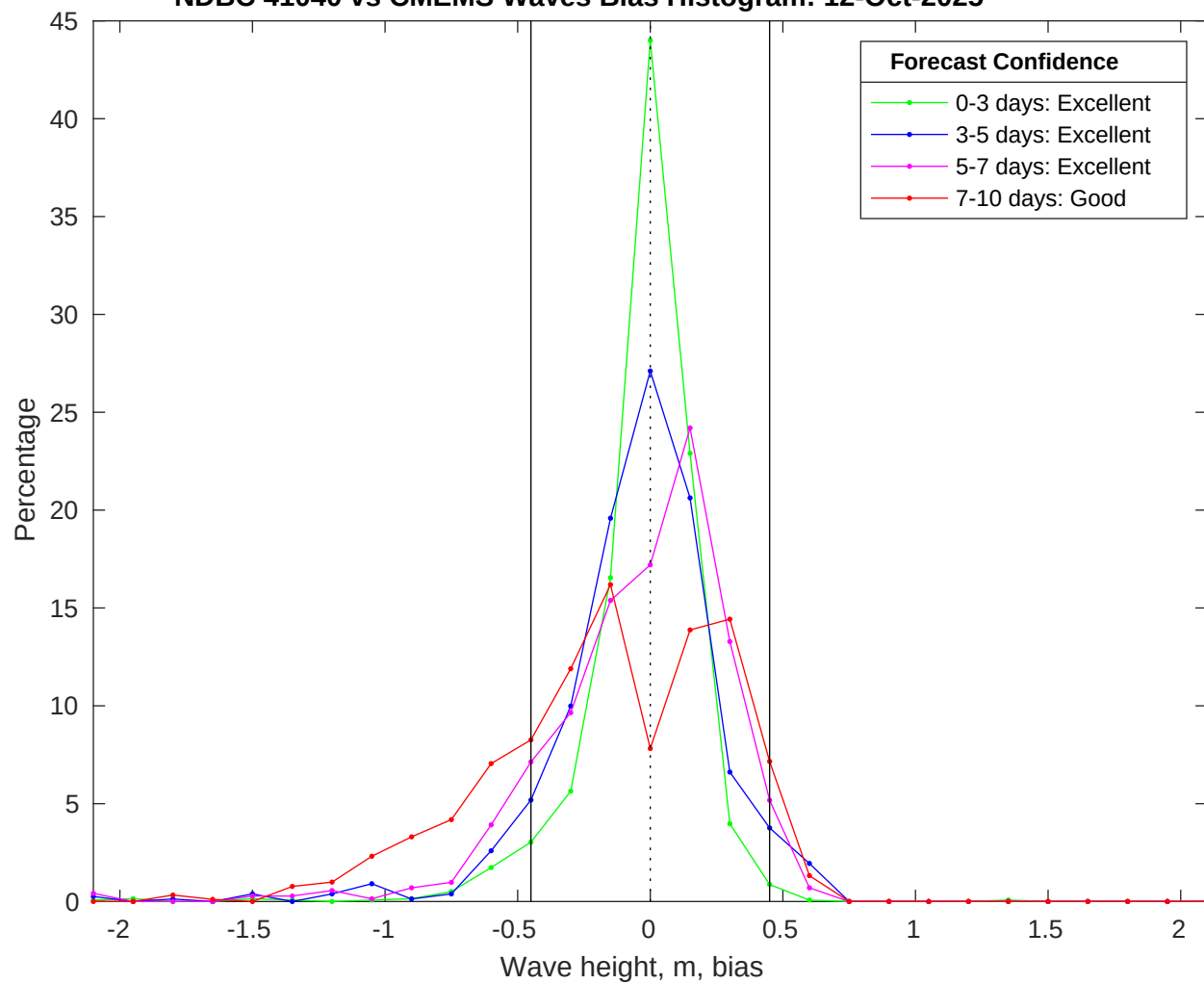
NDBC 41040 vs CMEMS Waves Bias Histogram: 12-Oct-2025
