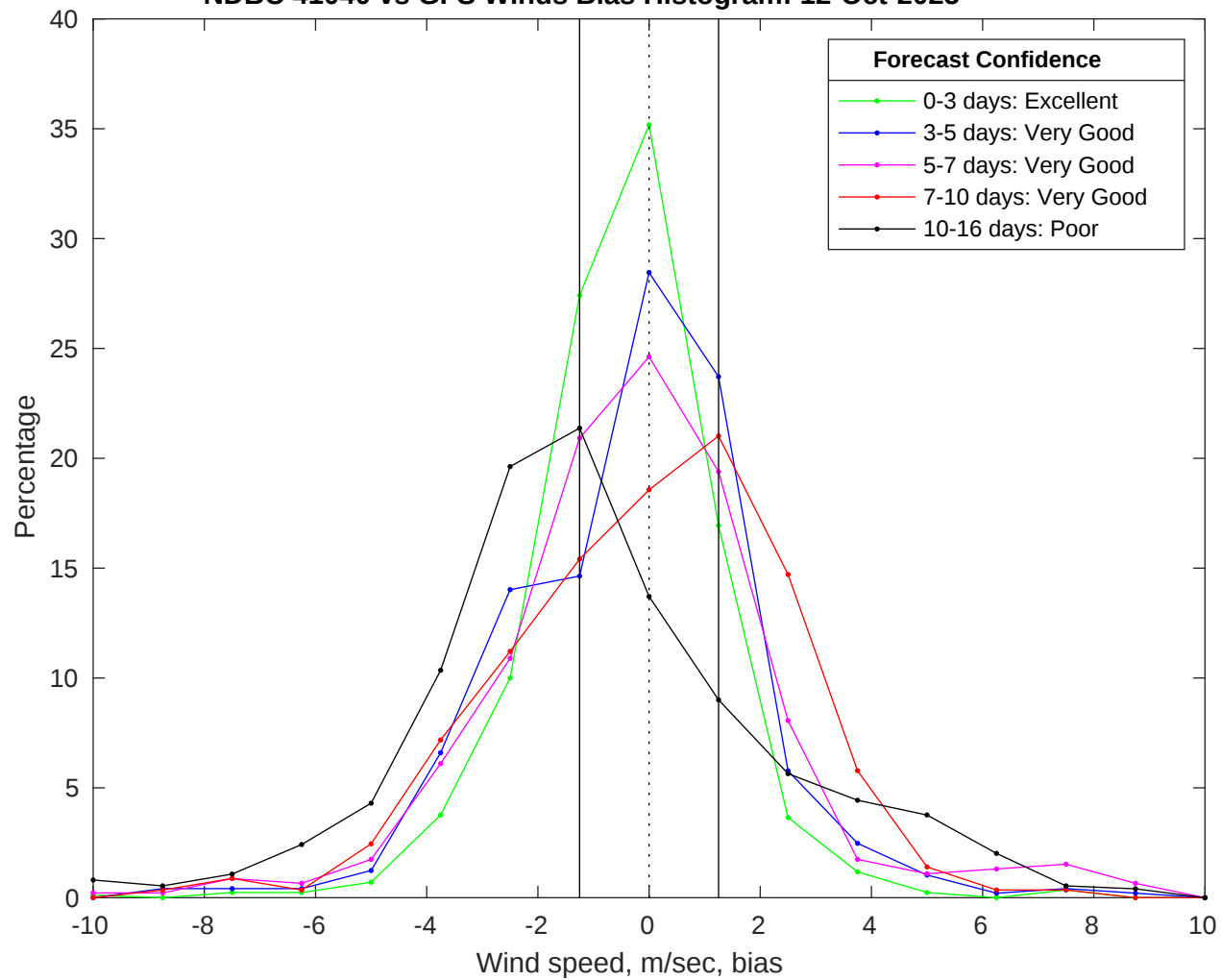
NDBC 41040 vs GFS Winds Bias Histogram: 12-Oct-2025
