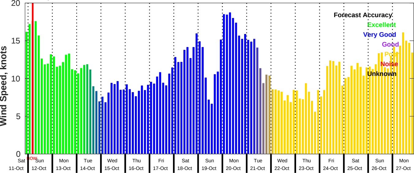
GFS Wind Speed Forecast for NDBC 41040 from 11-Oct-2025 21:00:00 to 27-Oct-2025 21:00:00
