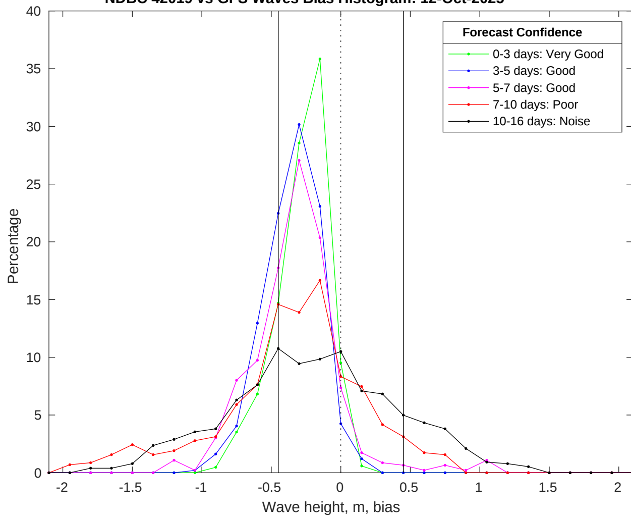
NDBC 42019 vs GFS Waves Bias Histogram: 12-Oct-2025
