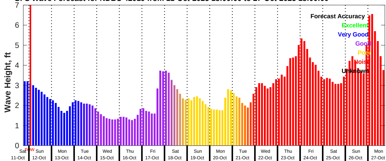
GFS Wave Forecast for NDBC 42019 from 11-Oct-2025 18:00:00 to 27-Oct-2025 18:00:00
