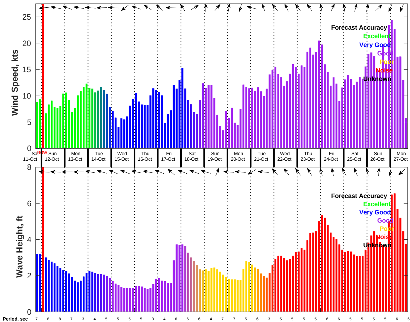
Wind & Wave Forecast for NDBC 42019 from 11-Oct-2025 18:00:00 to 27-Oct-2025 18:00:00
