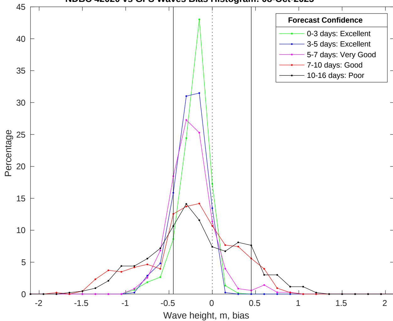
NDBC 42020 vs GFS Waves Bias Histogram: 08-Oct-2025
