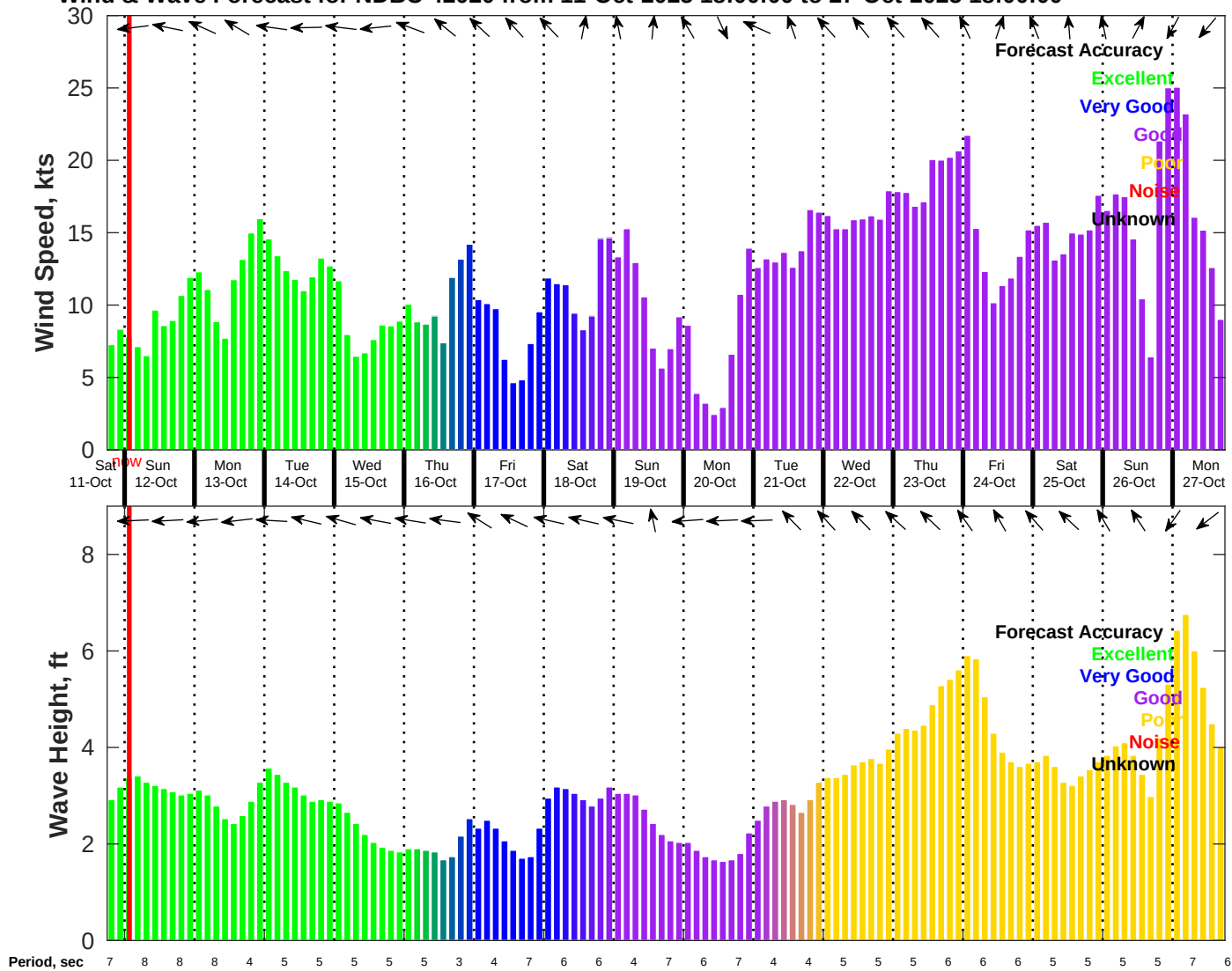
Wind & Wave Forecast for NDBC 42020 from 11-Oct-2025 18:00:00 to 27-Oct-2025 18:00:00
