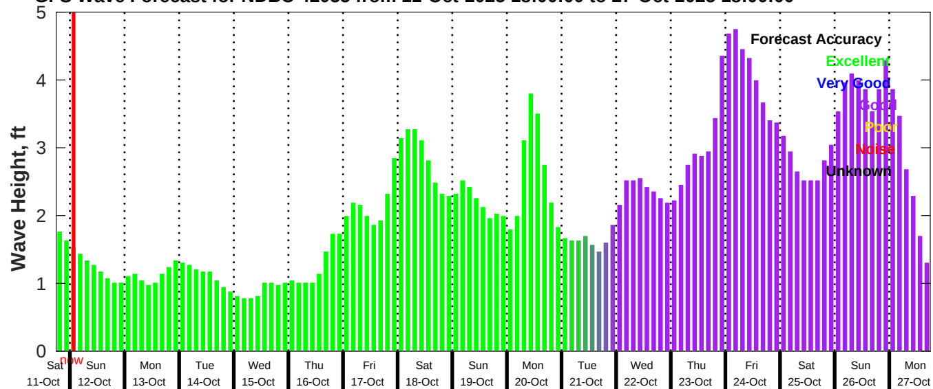
GFS Wave Forecast for NDBC 42035 from 11-Oct-2025 18:00:00 to 27-Oct-2025 18:00:00
