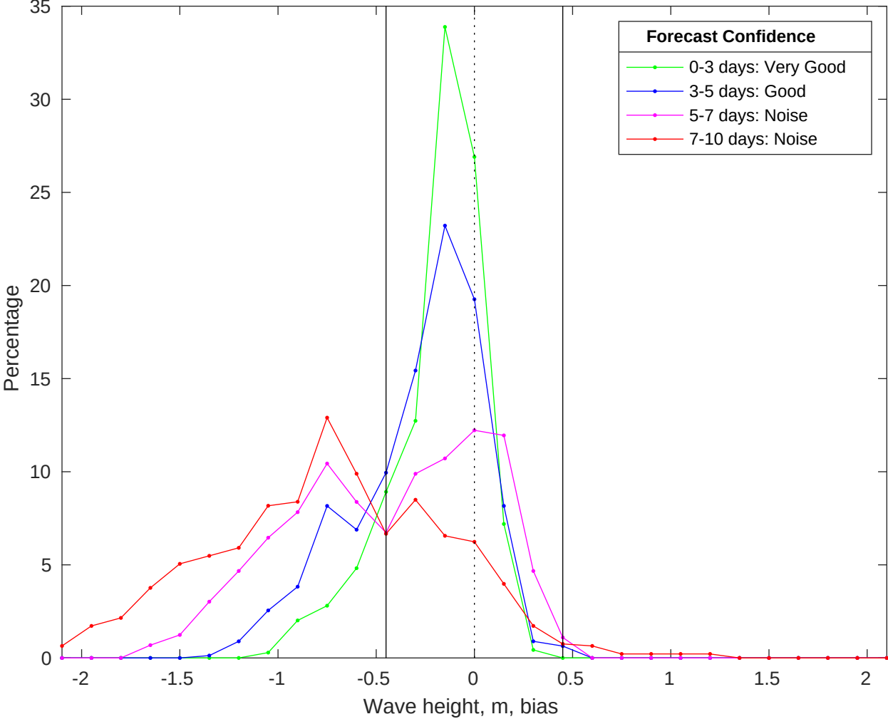
NDBC 42036 vs CMEMS Waves Bias Histogram: 12-Oct-2025
